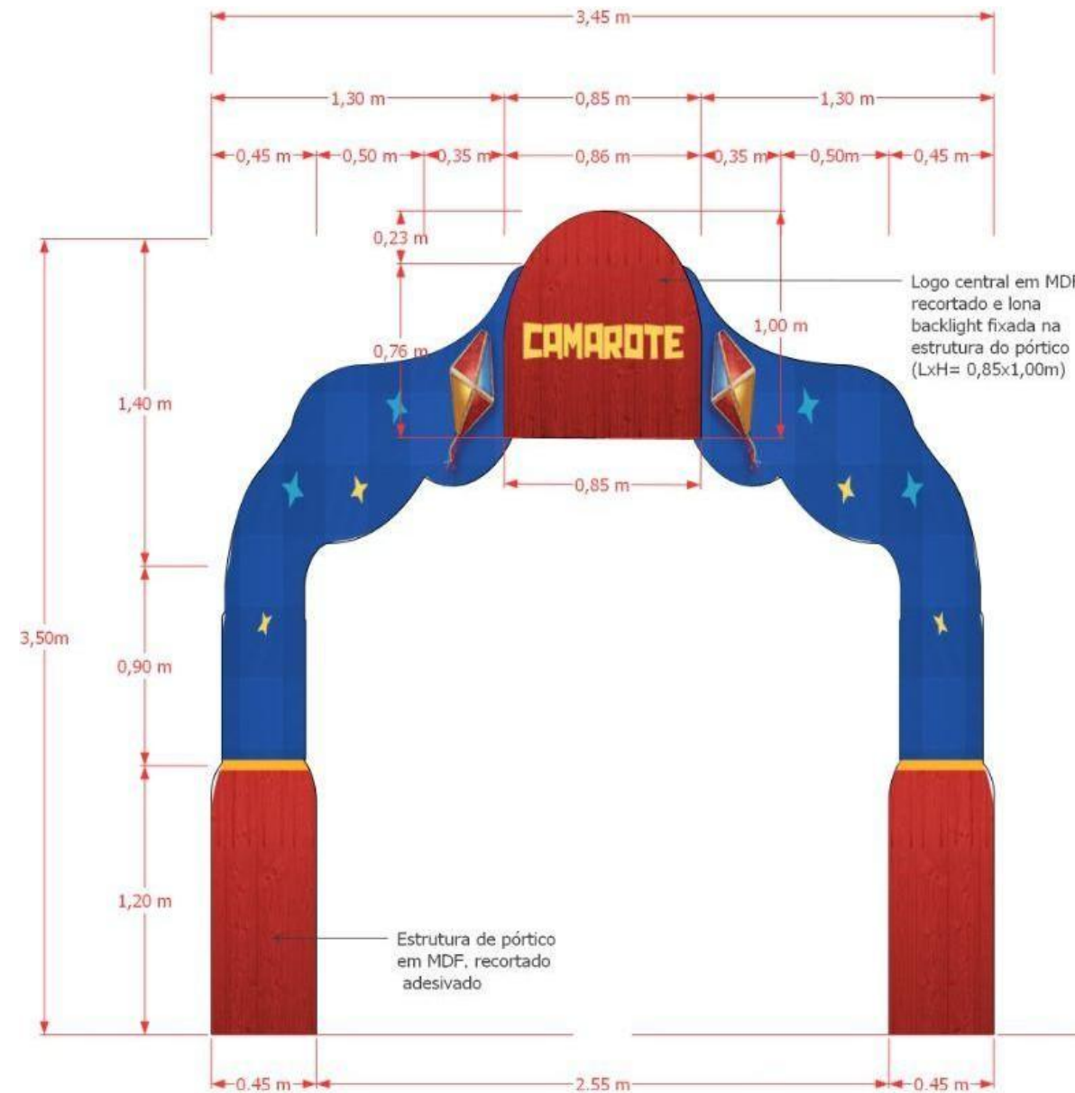
VISTA FRONTAL
