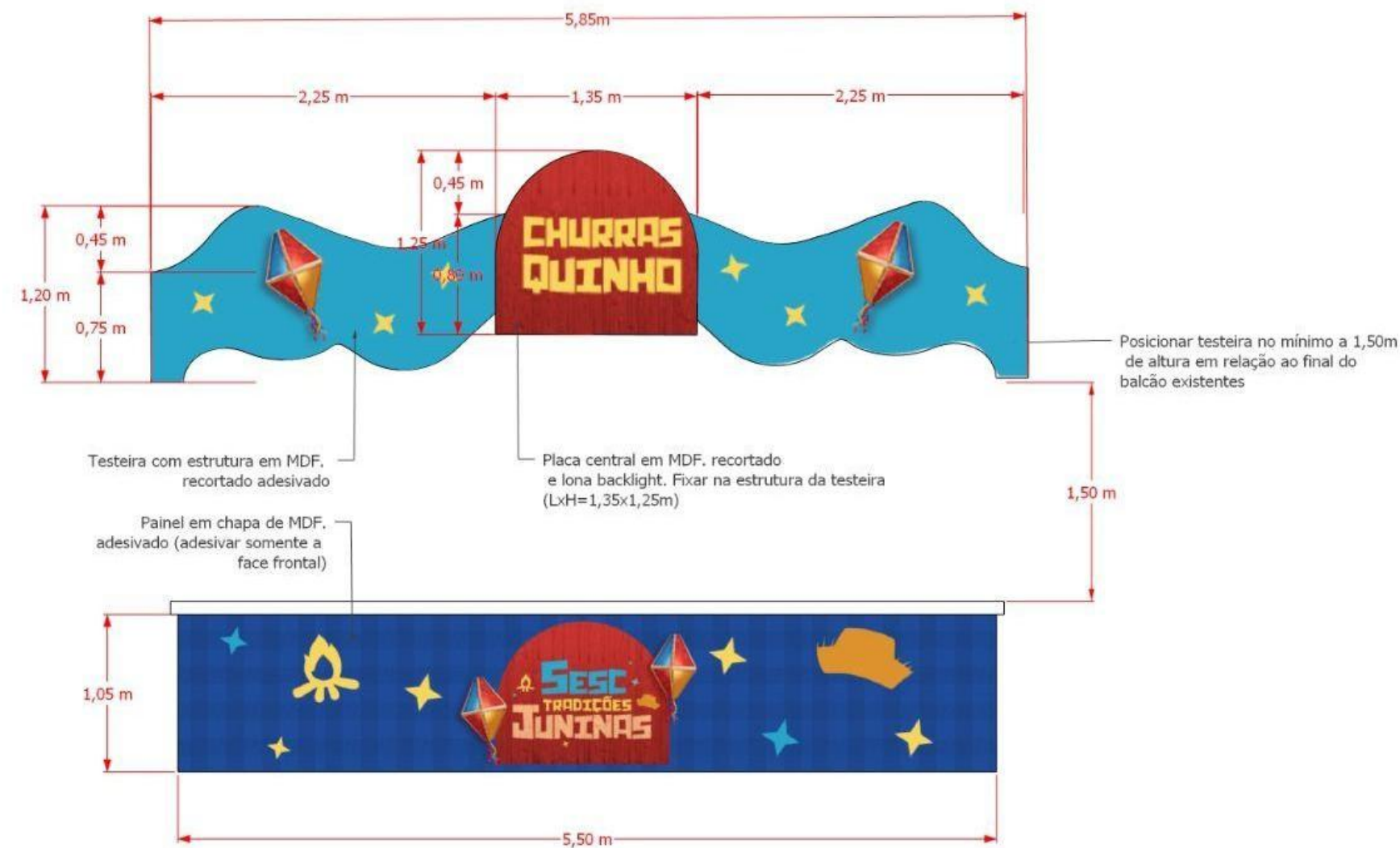
VISTA FRONTAL
