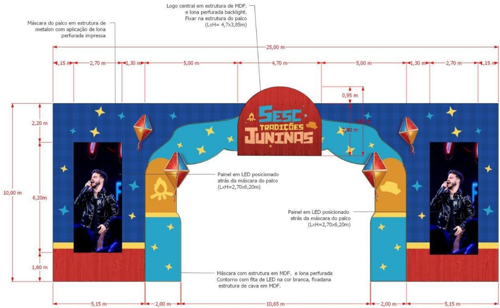
VISTA FRONTAL
