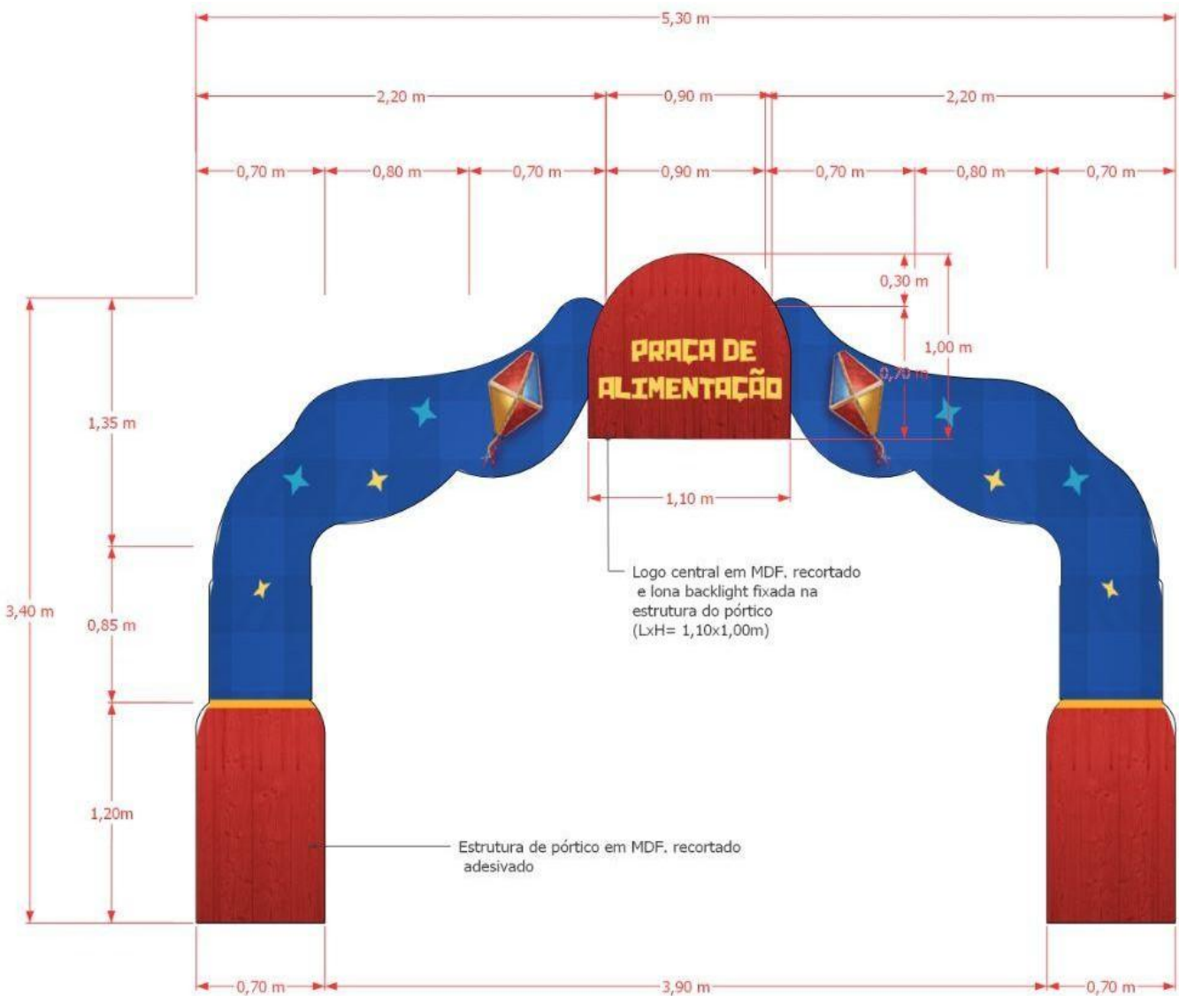
VISTA FRONTAL
